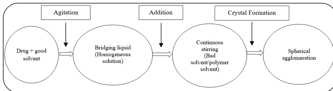
Figure 2. Crystallo-co-agglomeration technique
