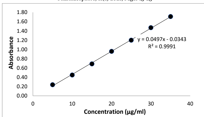
Figure 2. A plot of Absorbance versus Concentration of SEC ( \mu\text{g} )
