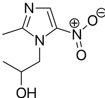
Figure 1. Chemical Structure of Secnidazole
