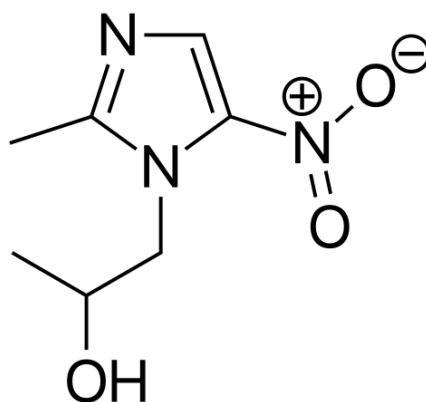
Figure 1. Chemical Structure of Secnidazole
