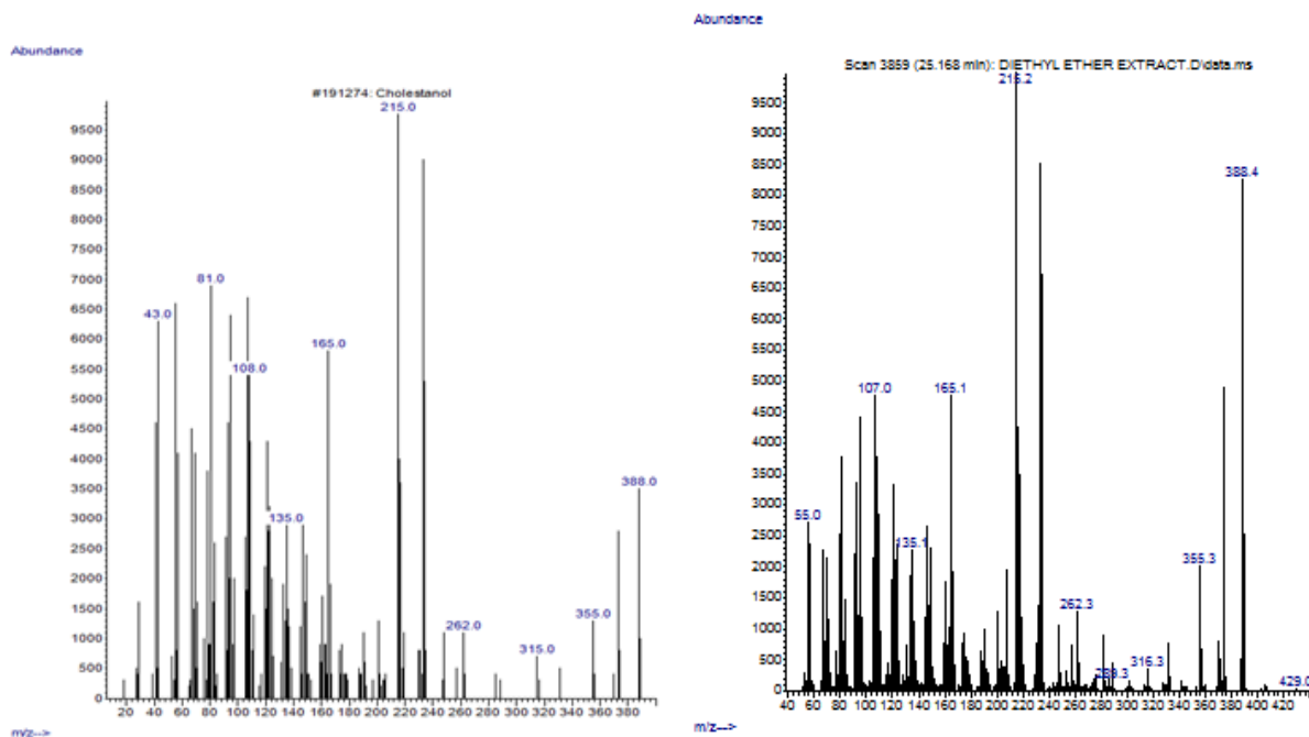
Figure 3. Mass spectrum of Haliclona sp. extract with RT=25.168 (right) and cholestanol reference (left)
