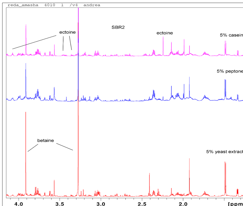
Figure 4. NMR ^1\text{H} spectra of cell extracts from Sediminibacillus sp. using yeast extract, peptone and casein in saline nutrient medium spectra spectra (Source Red Sea Sediment).
