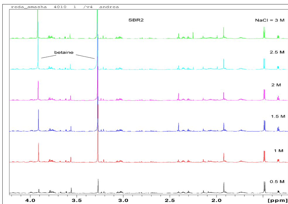
Figure 3. NMR 1 H spectra of cell extracts from Sediminibacillus sp. at 0.5, 1.0, 1.5, 2.0, 2.5 and 3.0 NaCl (M) in saline nutrient medium spectra (Source Red Sea Sediment).
