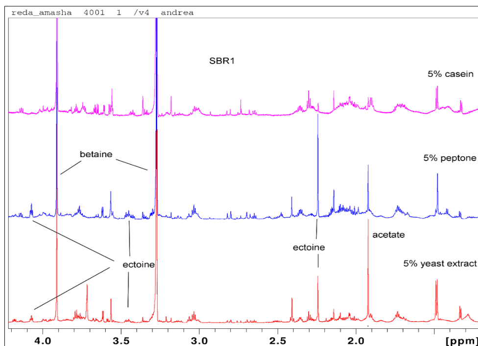
Figure 2. NMR 1 H spectra of cell extracts from Halomonas aquamarina using yeast extract, peptone and casein in saline nutrient medium spectra (Source Red Sea Sediment).
