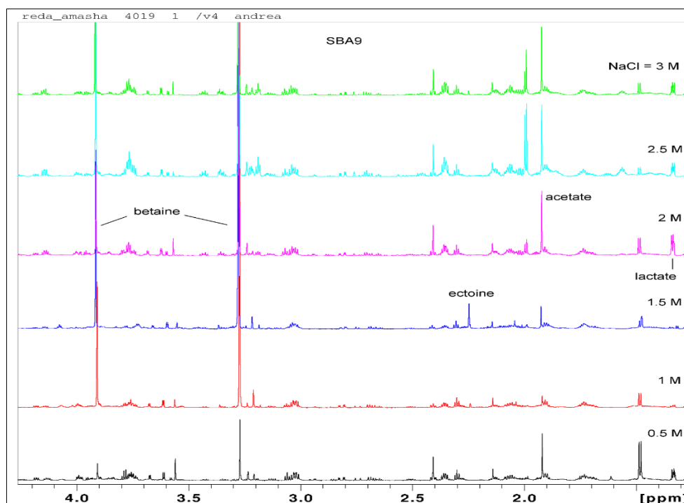
Figure 5. NMR ^1\text{H} spectra of cell extracts from Halobacillus sp. at 0.5, 1.0, 1.5, 2.0, 2.5 and 3.0 NaCl (M) in saline nutrient medium spectra (Source Arabian Sea water).
