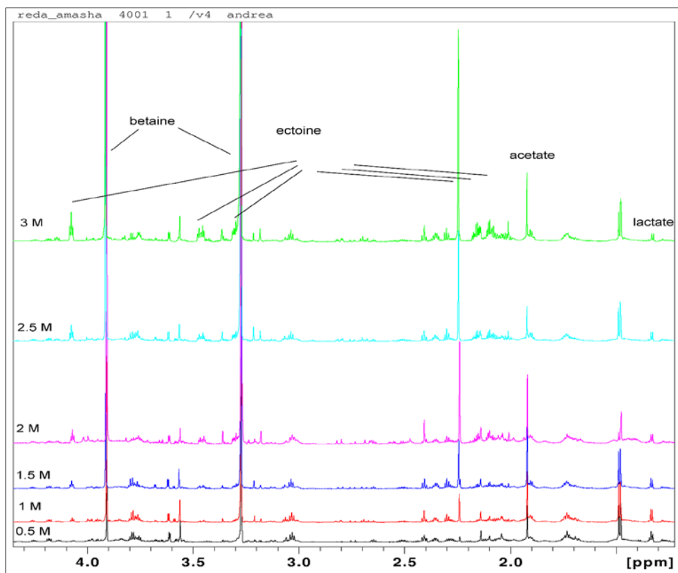
Figure 1: NMR ^1\text{H} spectra of cell extracts from Halomonas aquamarina at 0.5, 1.0, 1.5, 2.0, 2.5 and 3.0 NaCl (M) in saline nutrient medium spectra (Source Red Sea Sediment).
