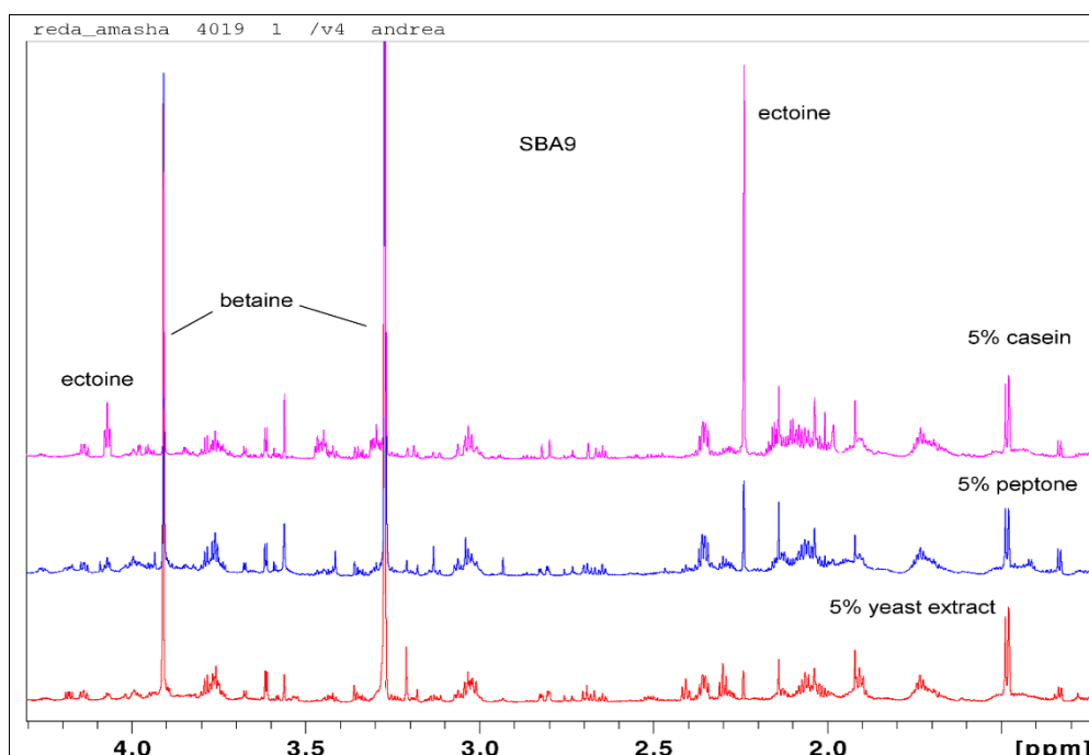
Figure 6. NMR ^1\text{H} spectra of cell extracts from Halobacillus sp. using yeast extract, peptone and casein in saline nutrient medium spectra (Source Arabian Sea water).
