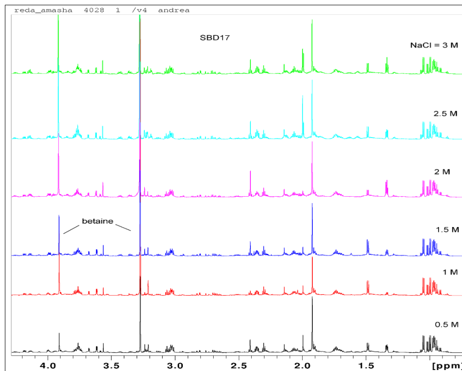
Figure 7. NMR 1 H spectra of cell extracts from H. dabanensis at 0.5, 1.0, 1.5, 2.0, 2.5 and 3.0 NaCl (M) in saline nutrient medium (Source Red Sea mud).
