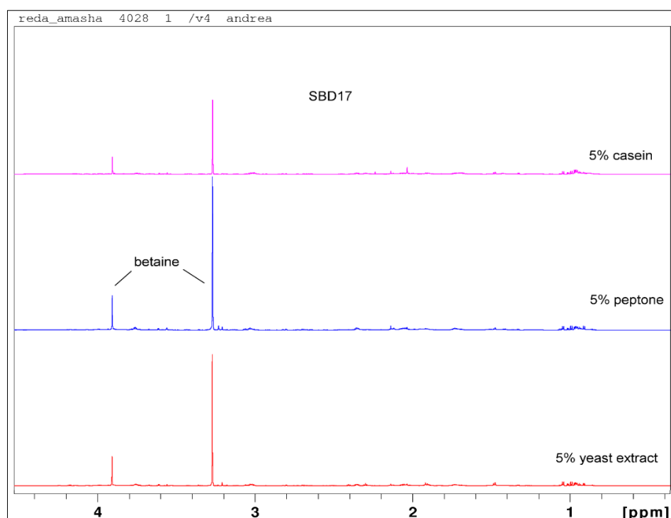
Figure 8. NMR 1 H spectra of cell extracts from H. dabanensis using yeast extract, peptone and casein in saline nutrient medium spectra (Source Red Sea mud).
